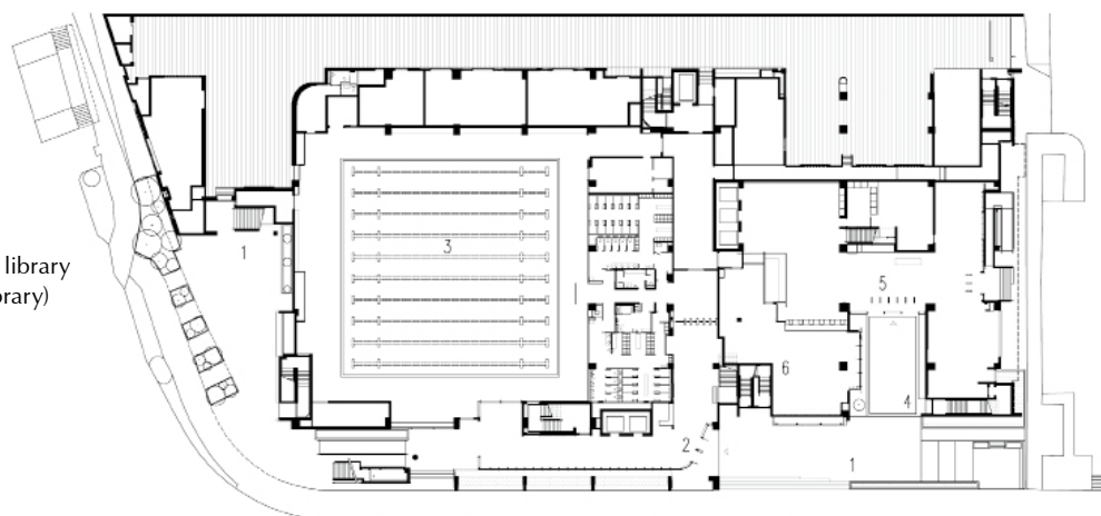
G/F floor plan
